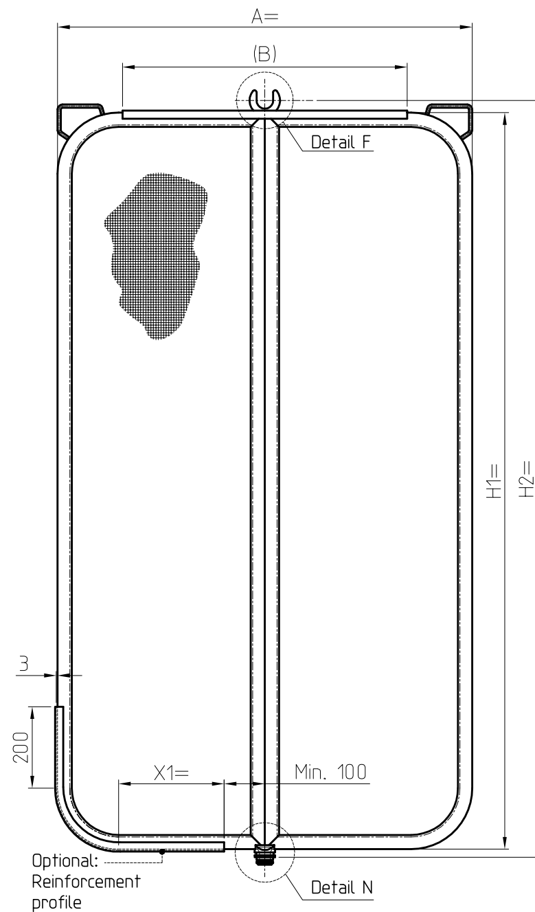
FILTERLEAF TYPE 2
