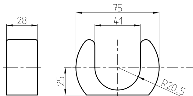
Standard dim. of fork (used by MAHLE)
