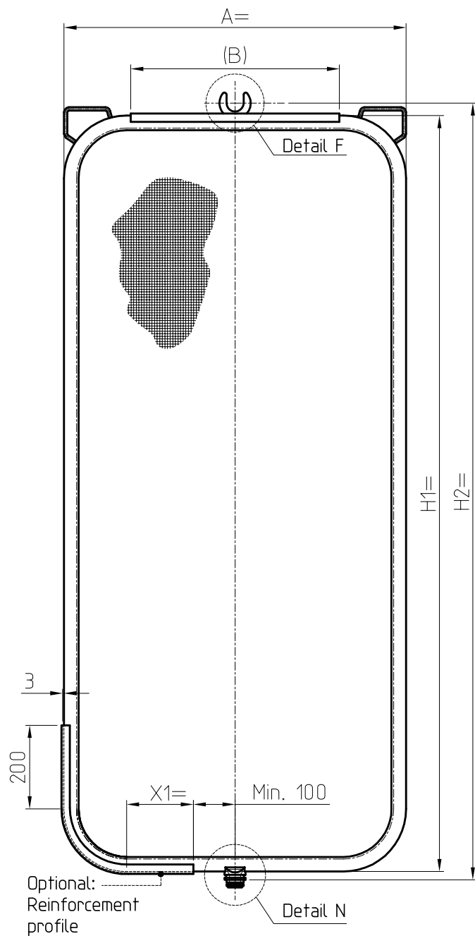
FILTERLEAF TYPE 1
