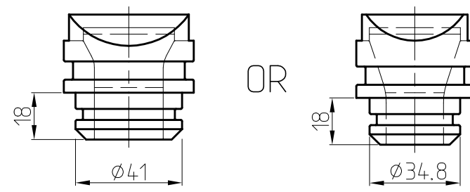
I Standard dim. of nozzle (used by MAHLE) II
